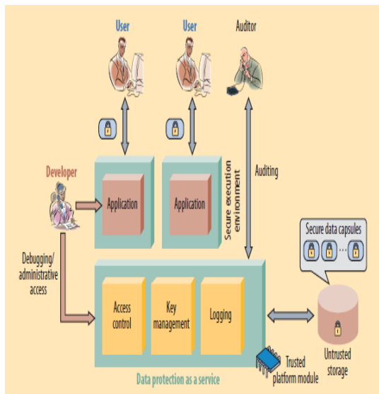
Fig. 2 –Architecture of DPaaS [19]
