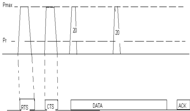
Figure .15. PCM periodically increases
