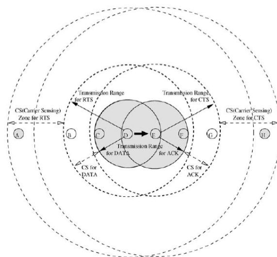
Figure .14. Basic Scheme.
