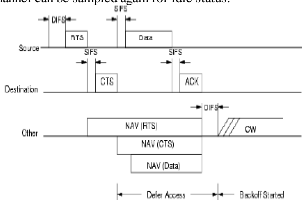
Figure 9. DCF access using RTS/CTS
