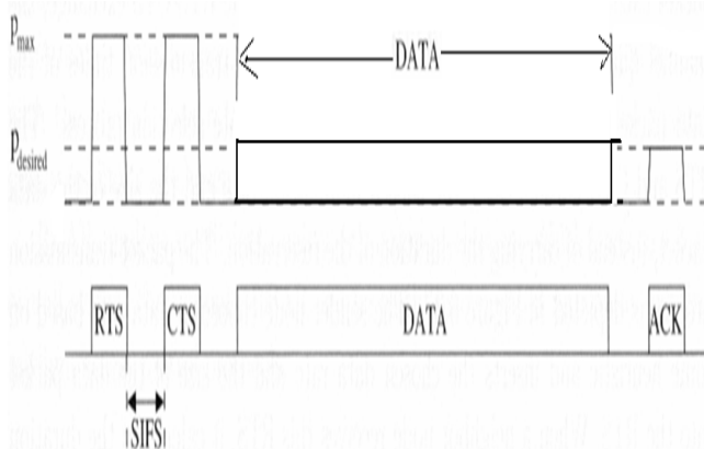
Figure .13. Basic Power Control Protocol.
