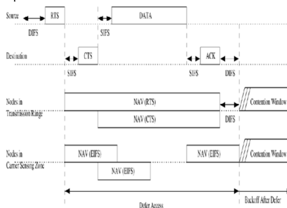
Figure 10. NAV duration in transmission range and carrier sensing zone
