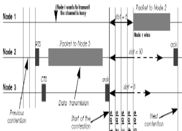
Figure .2. CSMA Channel Access Mechanism
