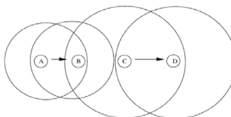
Figure 11. Differences in transmit power can lead to increased collisions
